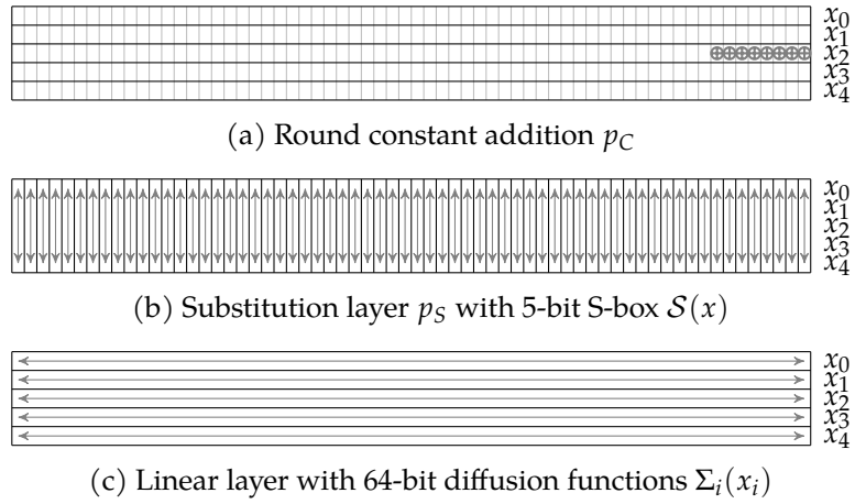
Figure 3: The register words of the 320-bit state S and operations p_L \circ p_S \circ p_C .
